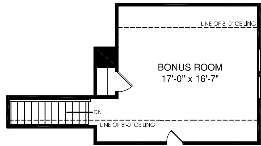
OPT. BONUS ROOM W/ OPT. MORNING ROOM
