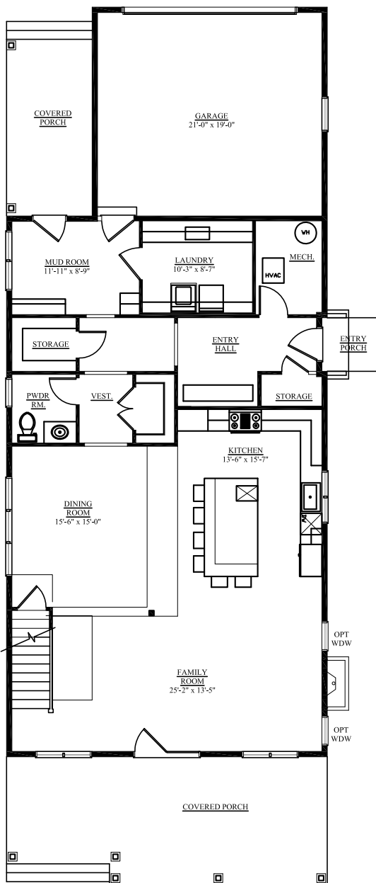
MAIN LEVEL FLOOR PLAN TWO CAR REAR GARAGE - GCD WITH OPTIONAL FULL PORCH - EPA
