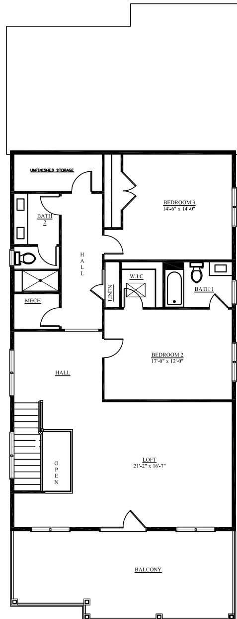
UPPER LEVEL PLAN OPT. 3 BEDROOM W/ LOFT - GCS WITH OPTIONAL FULL PORCH - EPA
