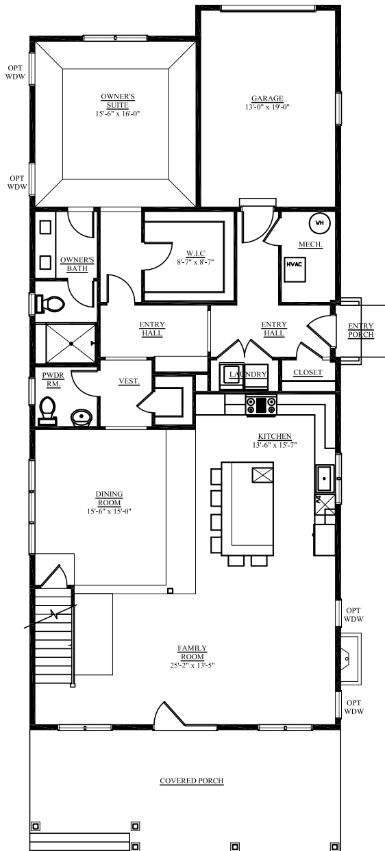
MAIN LEVEL FLOOR PLAN ONE CAR REAR GARAGE - GCS WITH OPTIONAL FULL PORCH - EPA
