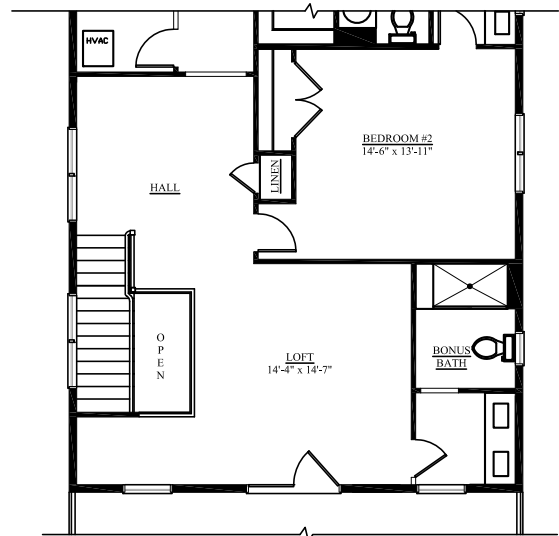
PARTIAL UPPER LEVEL PLAN OPT. BATHROOM W/ SHOWER - ABA WITH OPTIONAL FULL PORCH - EPA
